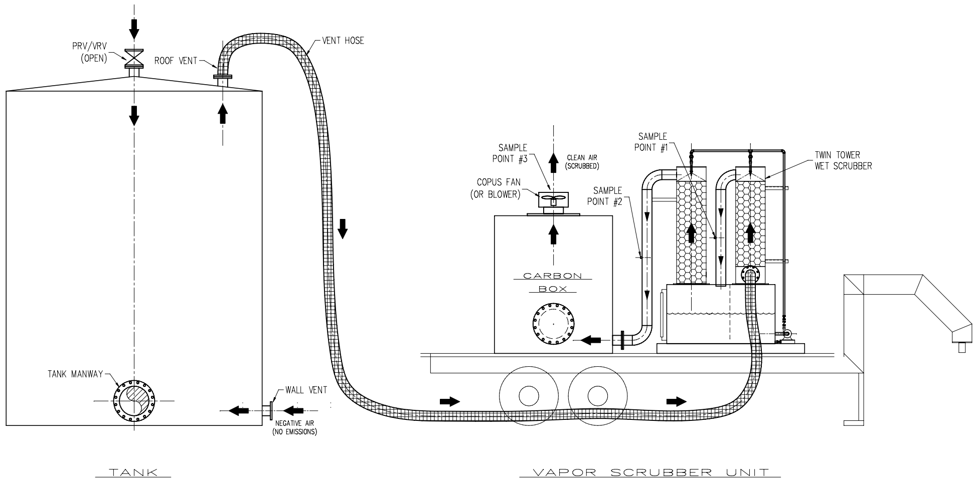
BASIC SCRUBBER SYSTEM SETUP DURING TANK CLEANING & DEGASSING OPERATIONS (REVISION 'B' 3-24-09)
